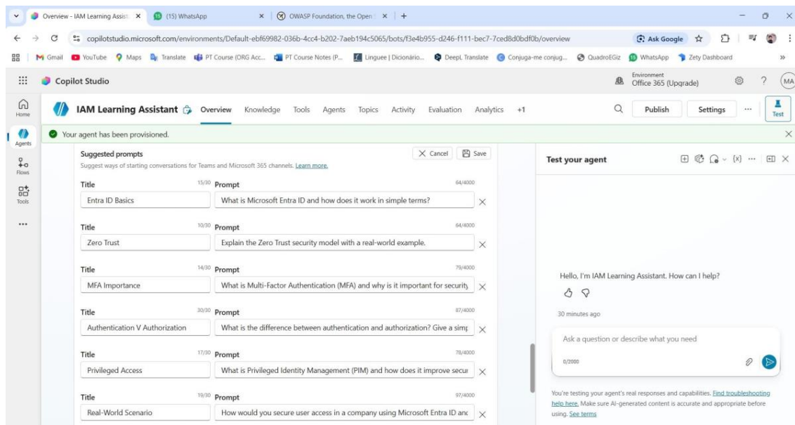
Image 5: prompts
