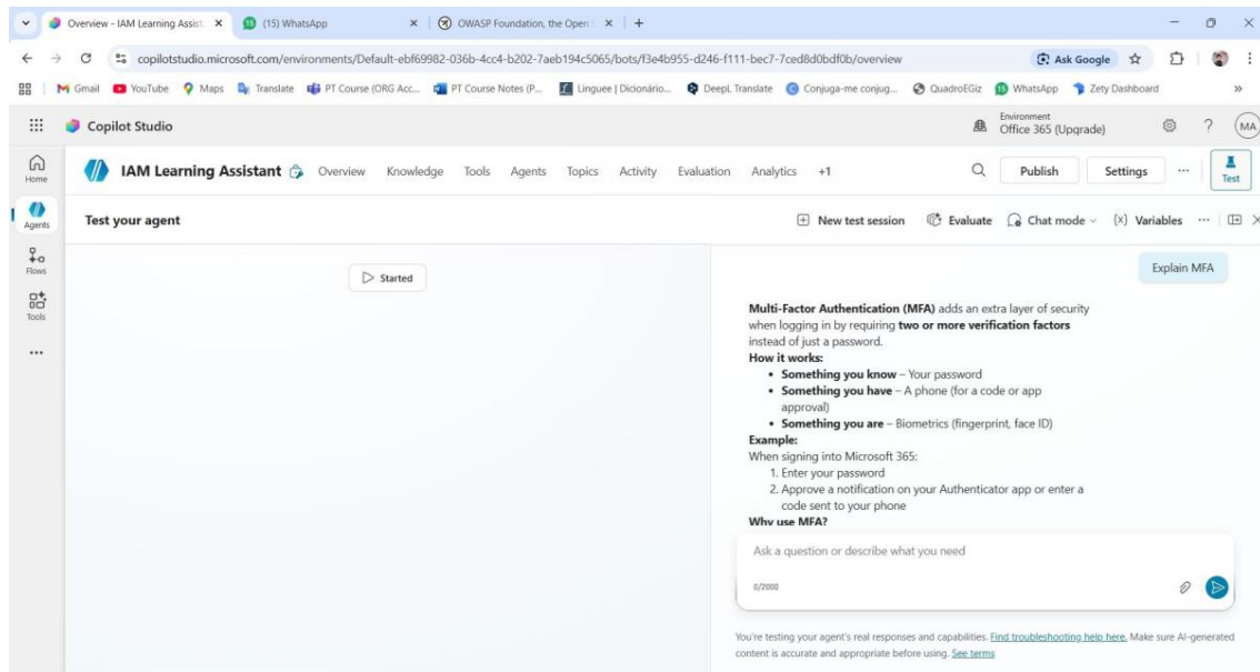
Image 6: Example response
