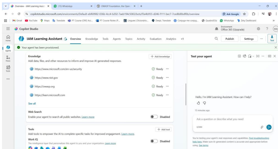
Image 4: Knowledge sources
