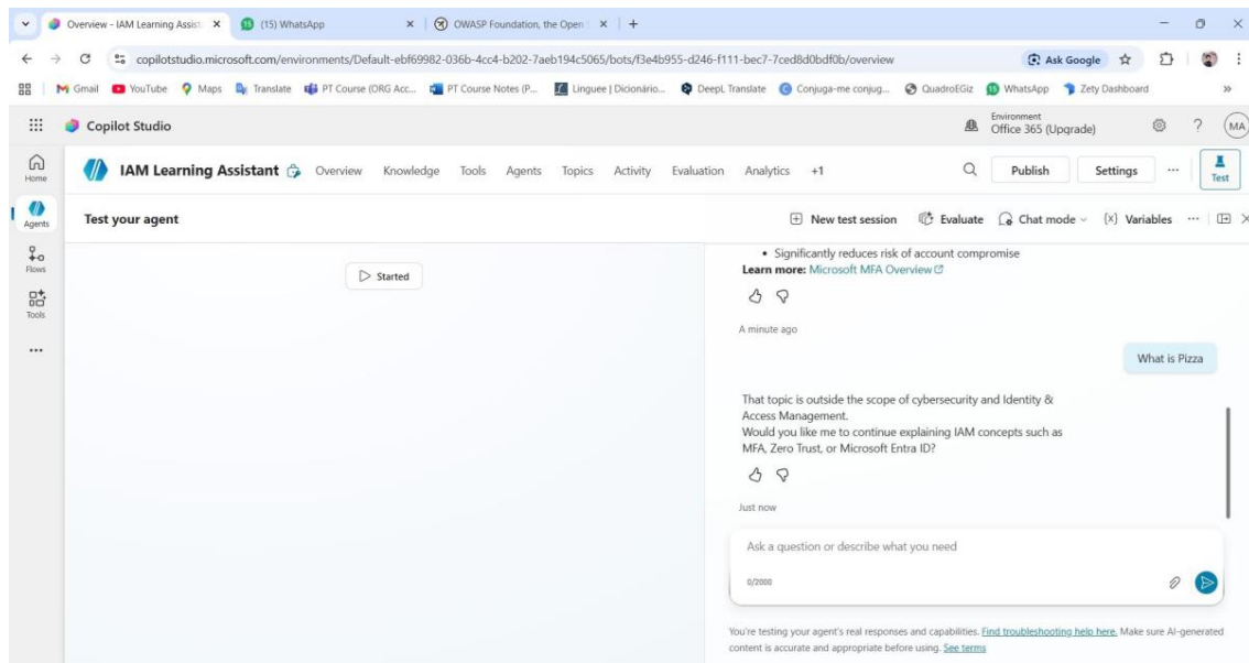
Image 7: Irrelevant query
