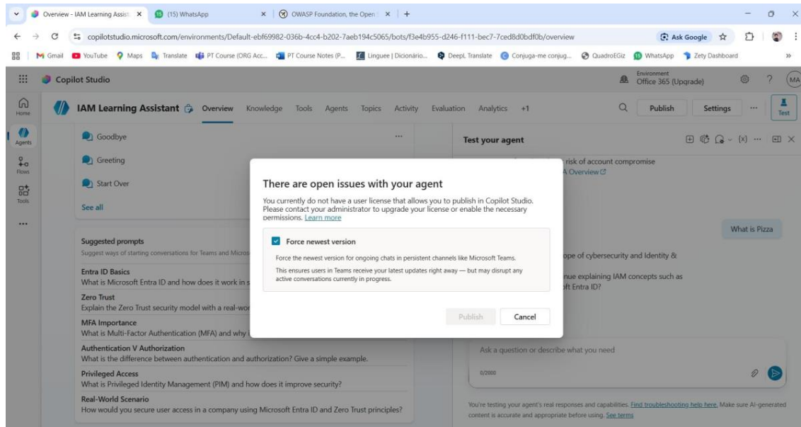
Image 8: License error
