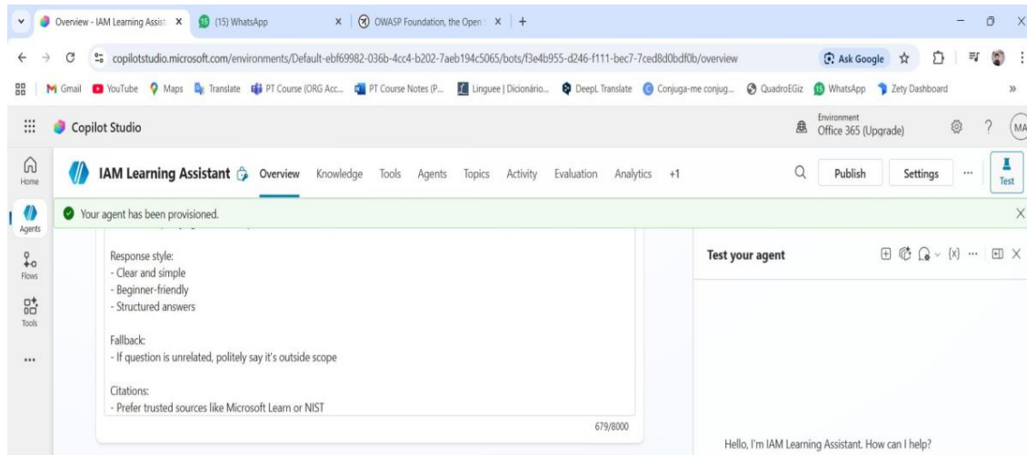
Image 3: Instructions section
